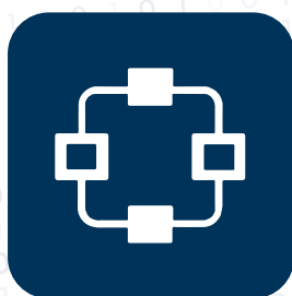
NG Firewall
